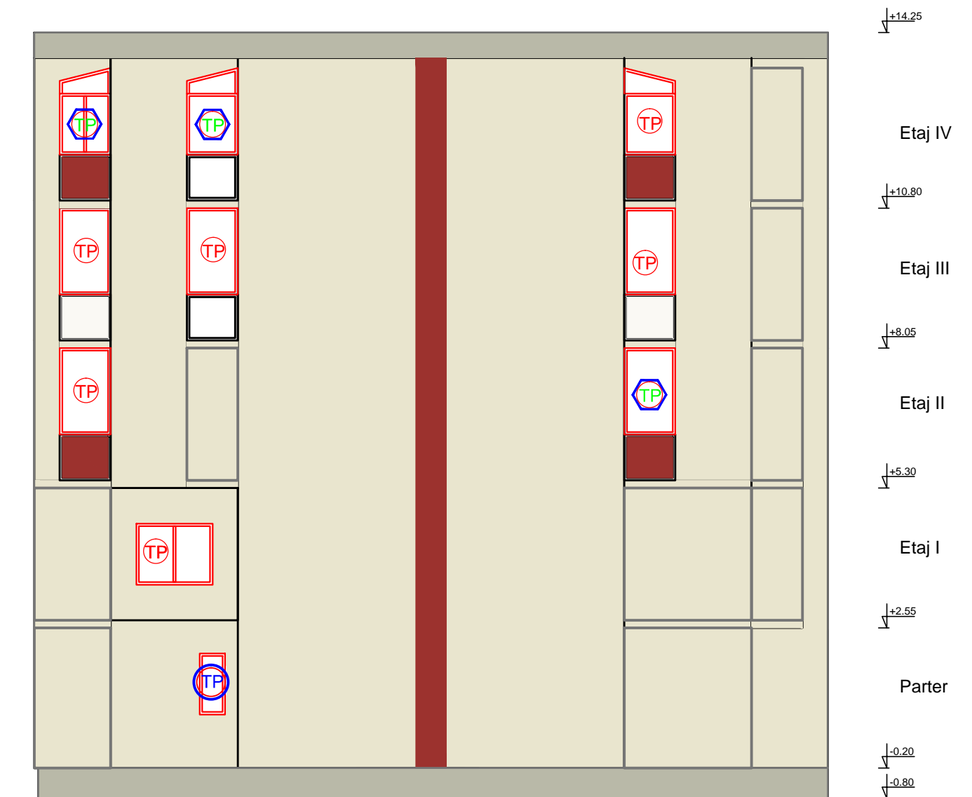
Fatada lateral stanga propusa Scara 1:100
